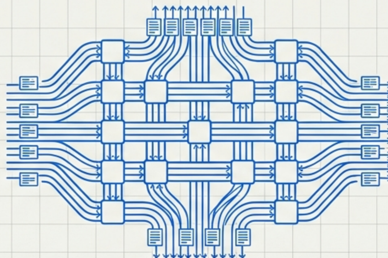
AGENTIC MODEL
