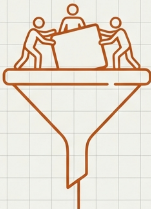
TRADITIONAL MODEL
